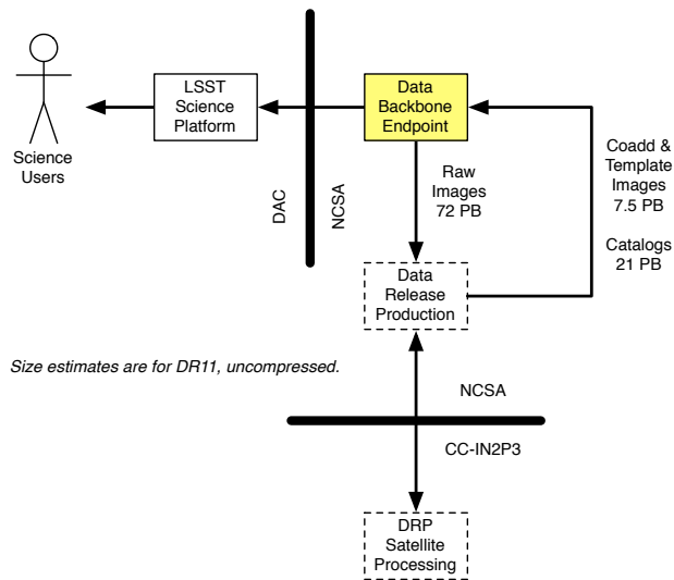
FIGURE 3: Annual Reprocessing Data Flows
