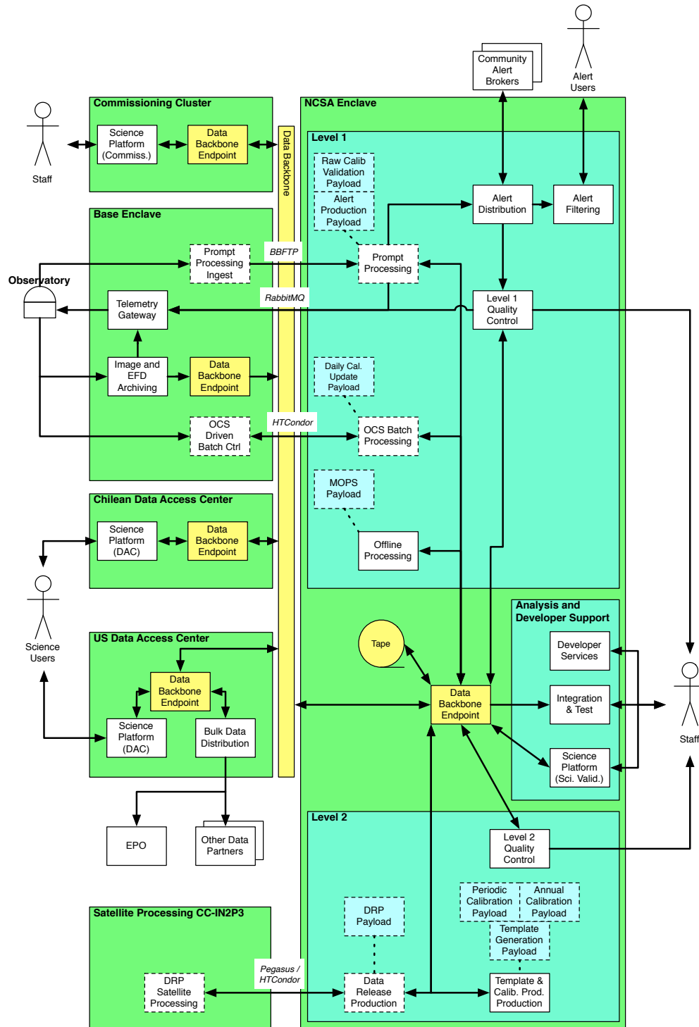
FIGURE 4: Data Management System Deployment
