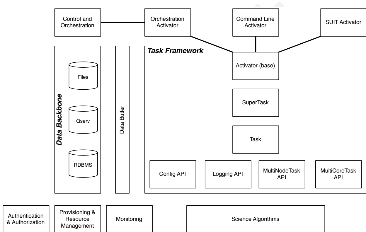
FIGURE 7: Data Management Middleware and Infrastructure
