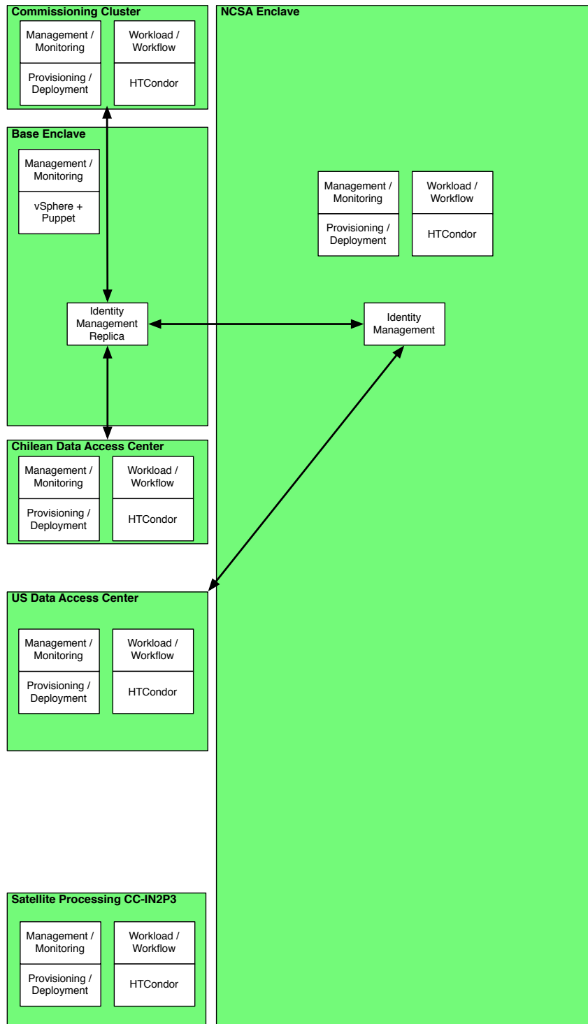
FIGURE 5: Data Management System Common Infrastructure Services
