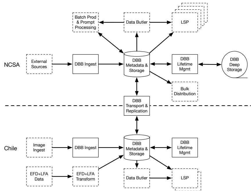
FIGURE 8: Data Backbone
