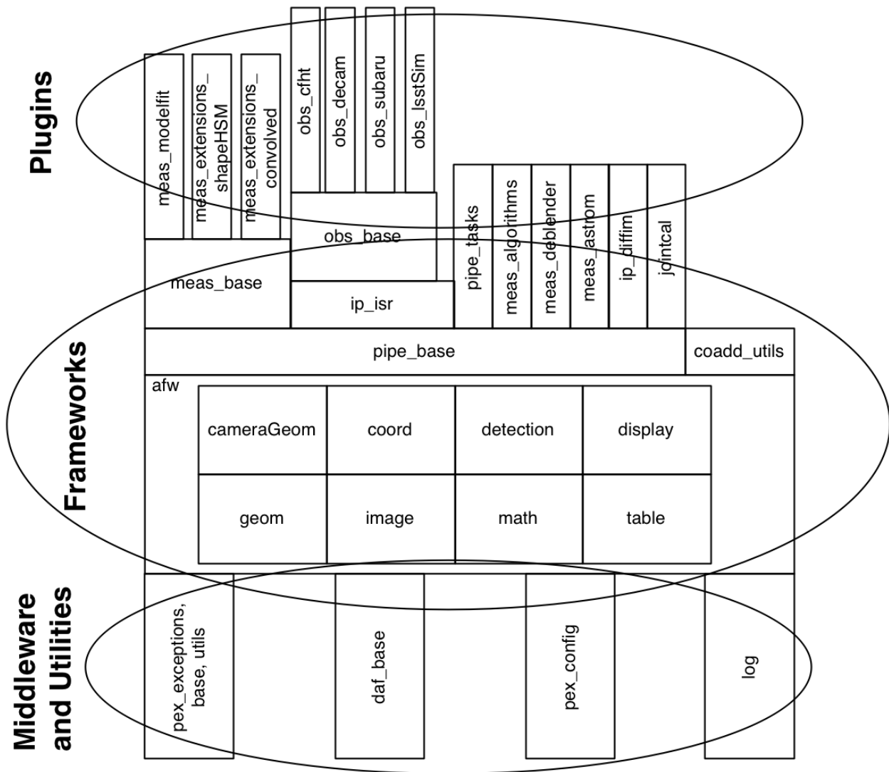
FIGURE 5: Data Management Science Pipelines Software “Stack”
