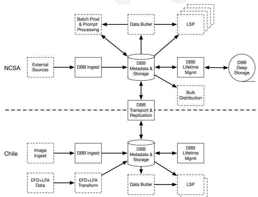
FIGURE 8: Data Backbone
