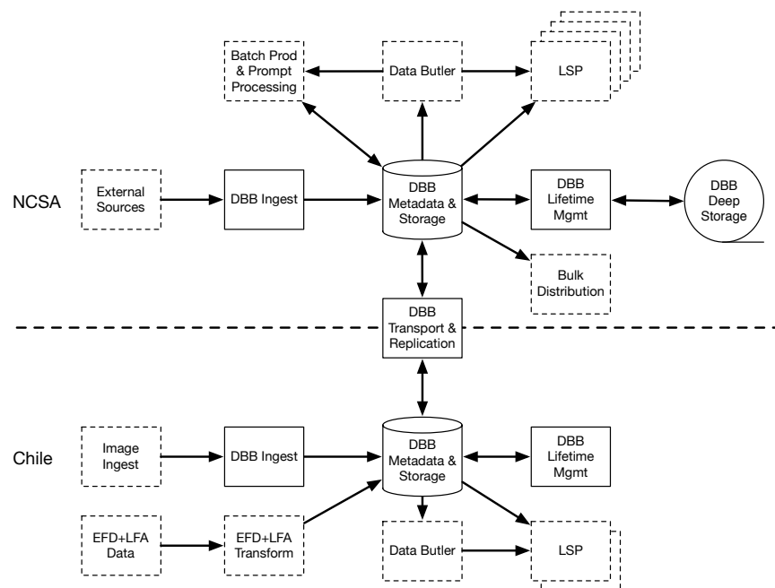
FIGURE 7: Data Backbone
